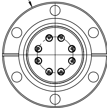
VACUUM SIDE CONNECTOR
