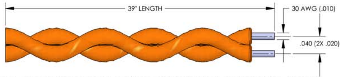
Kapton Insulated In-Vacuum Wire, Solid Core, Thermocouple Pair (Twisted), Type-K, 30 AWG, 39" length
